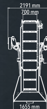
Dimensions conveyor belt FB5
