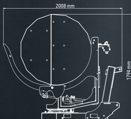
Dimensions 3-point bundler eco & proline, 1,0 rm
