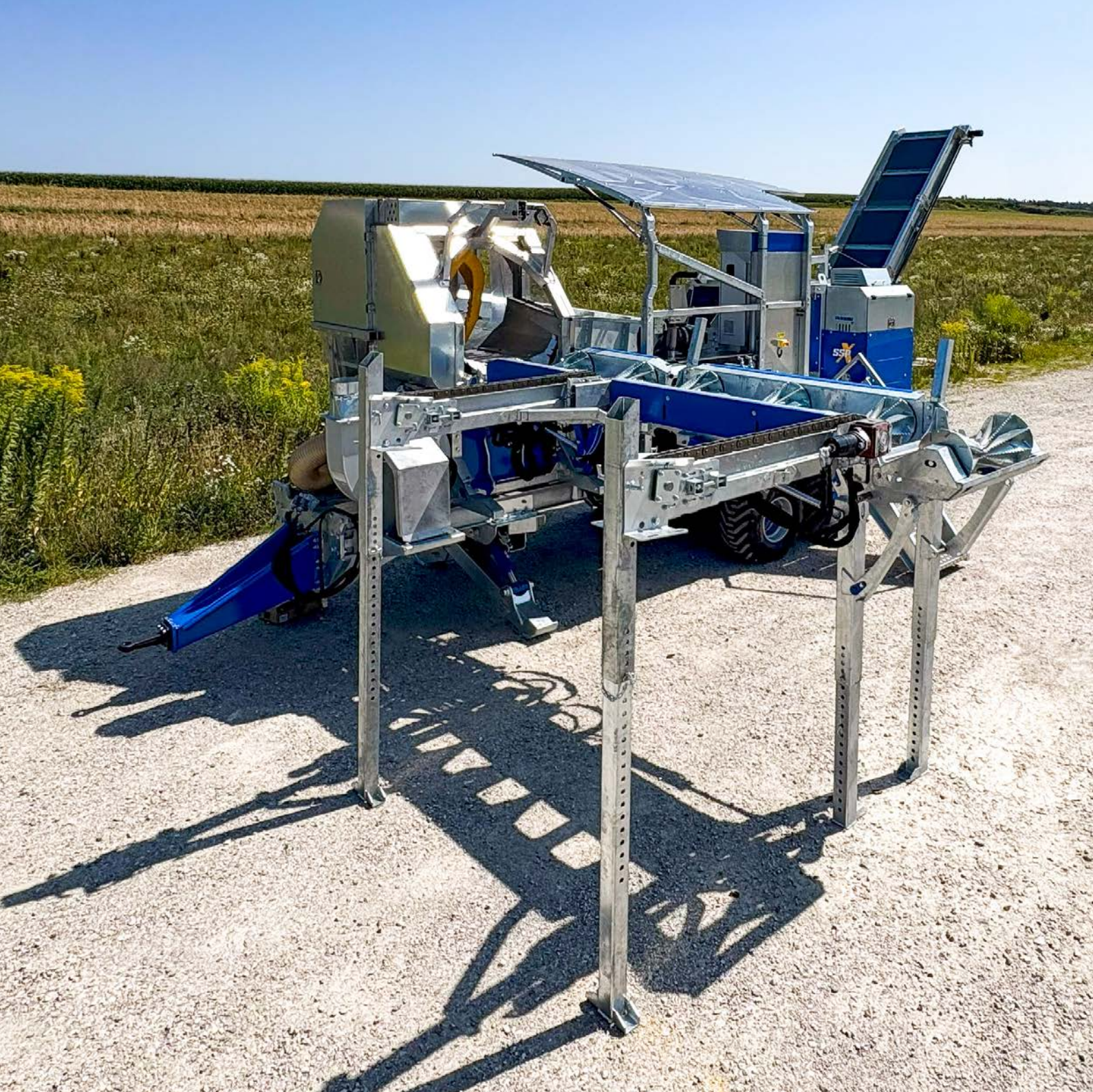
Cutting Unit
