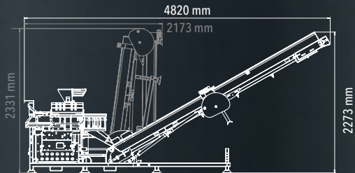
Dimensions conveyor belt 4 m
